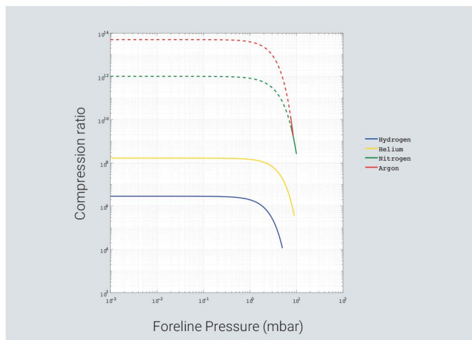
Compression Ratio
