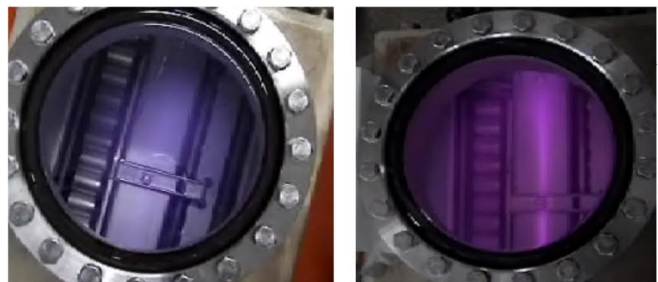
Figure 5. Diode element. For voltages below approximately 1 kV, the discharge is not confined, but it is extended to the entire pump volume.
