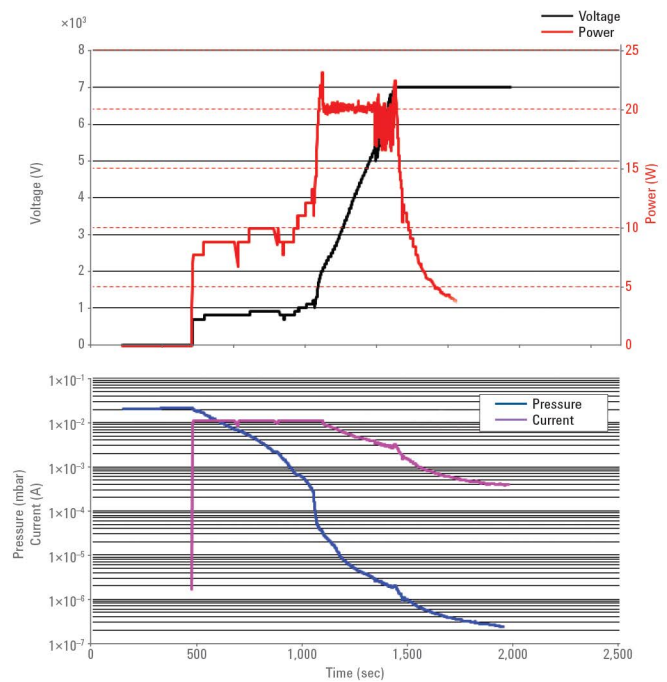
Figure 6. StarCell element, no gas flux, starting pressure 2 \times 10^{-2} mbar, 20 W maximum power. After approximately 8 minutes at 900 V, where the pumping is poor since only ions implanted in the cathode are pumped, the pumping efficiency increases as V increases, since gas is also pumped at the anode due to cathode sputtering. Maximum voltage was achieved approximately 16 minutes after the voltage was switched on.
