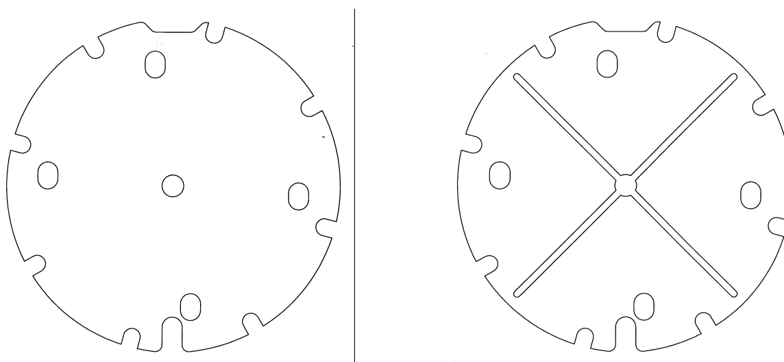
Figure A-3 Solid Steel and Slotted Stainless Clamp Plate
