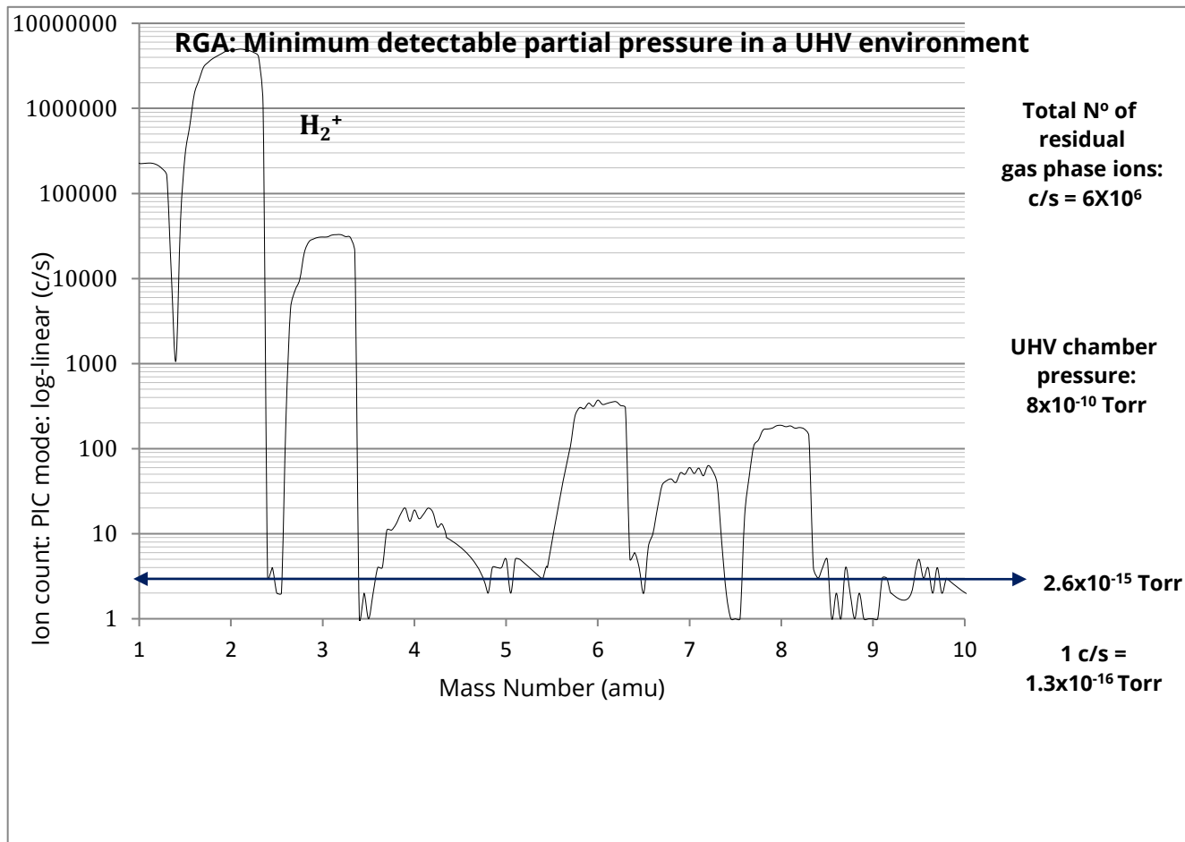
Figure1. Minimum Detectable Partial Pressure in a UHV environment
