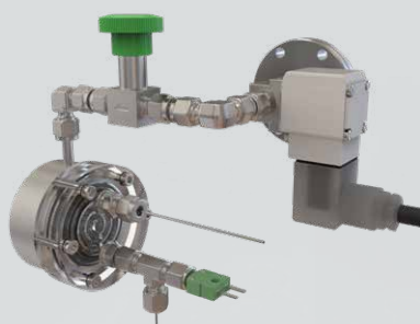
X44 Inlet Assembly
