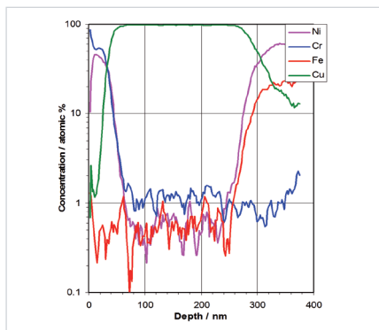
SNMS - Hard disk head layer structure
