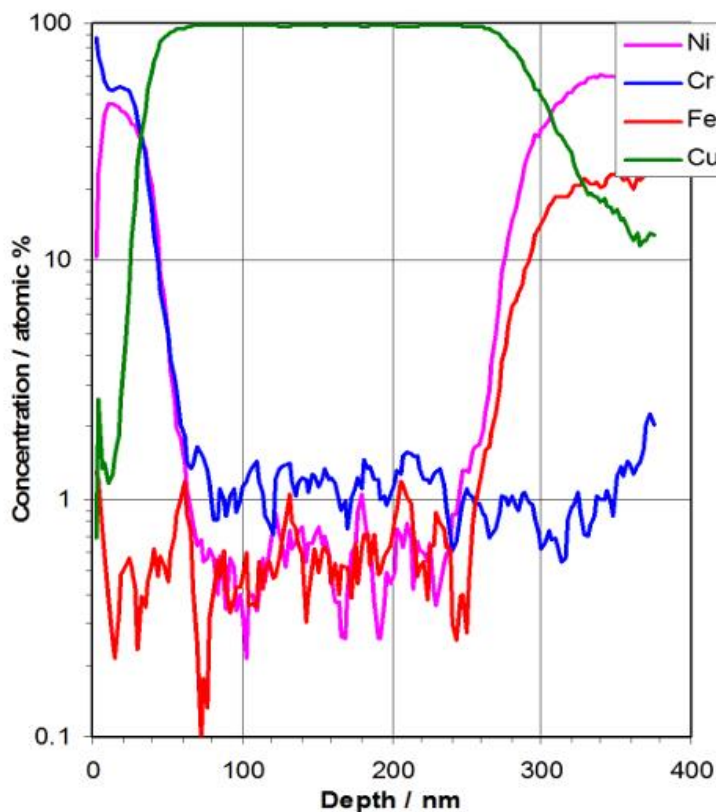
SNMS depth profile through magnetic layer stack
